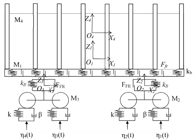
Fig. 4. Estimation scheme of the platform car with a removable module
